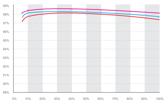
Growatt CP850TL-S 效率曲線 Growatt CP850TL-S efficiency
